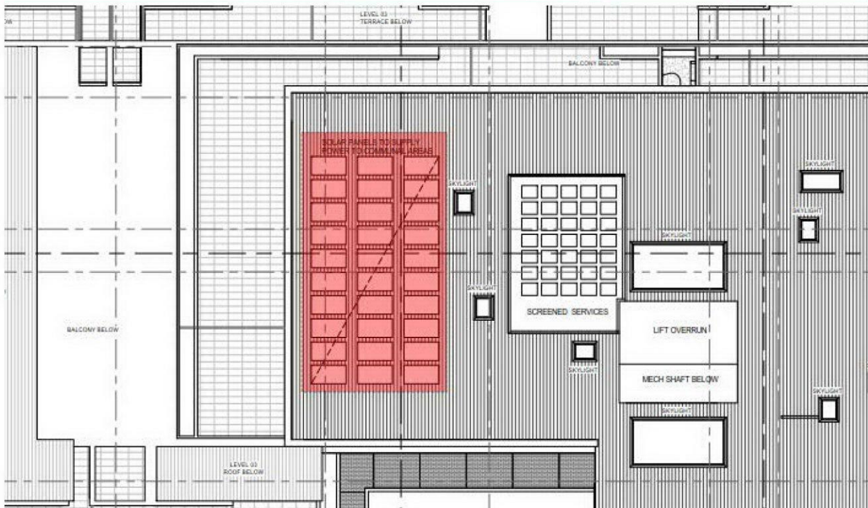
Figure 5: Proposed location of 10.0kW Solar PV System
