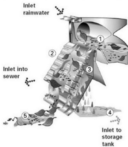
Figure 13: Cross-section of example filtration device before rainwater tank - Rainceptor (Source: AKS Industries)
